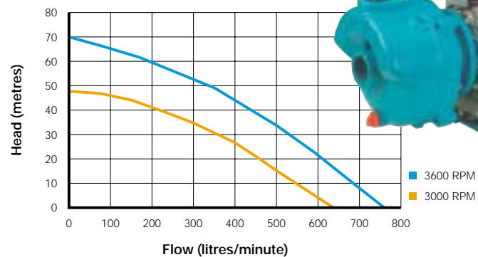
384 Hi-Flo Performance
