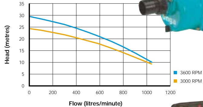
GP960 Performance
