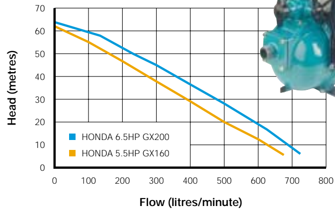
Blazemaster Performance
