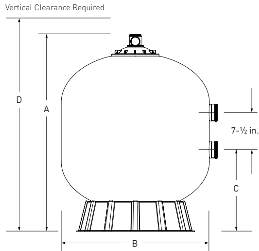
DIMENSION TABLE
